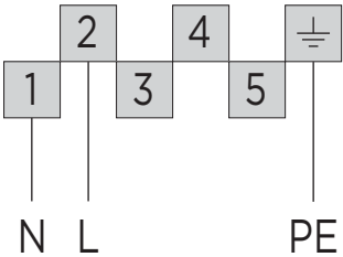
Single-phase connection (220-240 V~)
